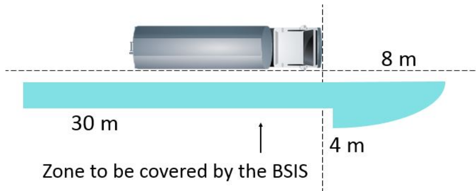
Figure 3 - Coverage required to pass the test protocol from UNECE
